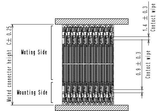
Mating Cross Section(FREE)
