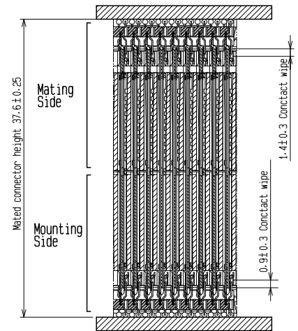
Mating Cross Section (Free)
